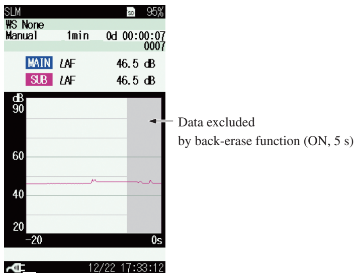
Time-Level screen
